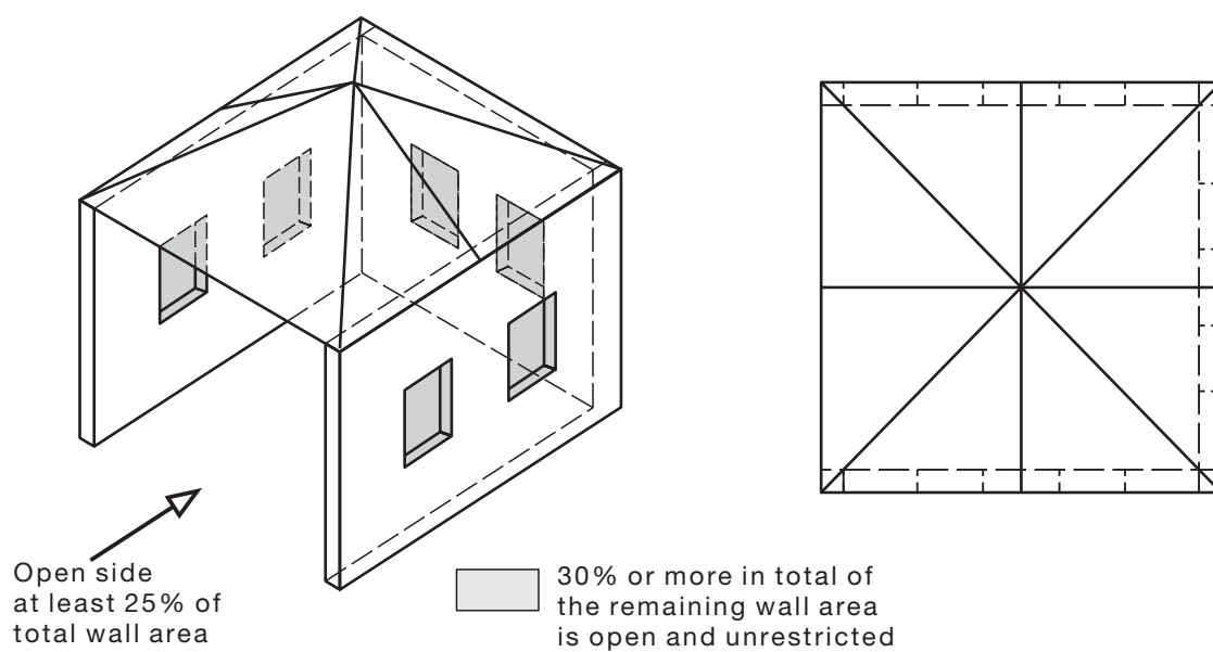
FIGURE 15 OUTDOOR AREA—EXAMPLE 5
